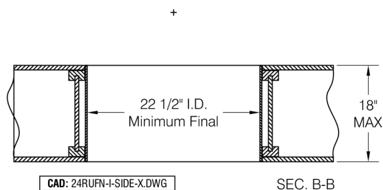
SEC. B-B
